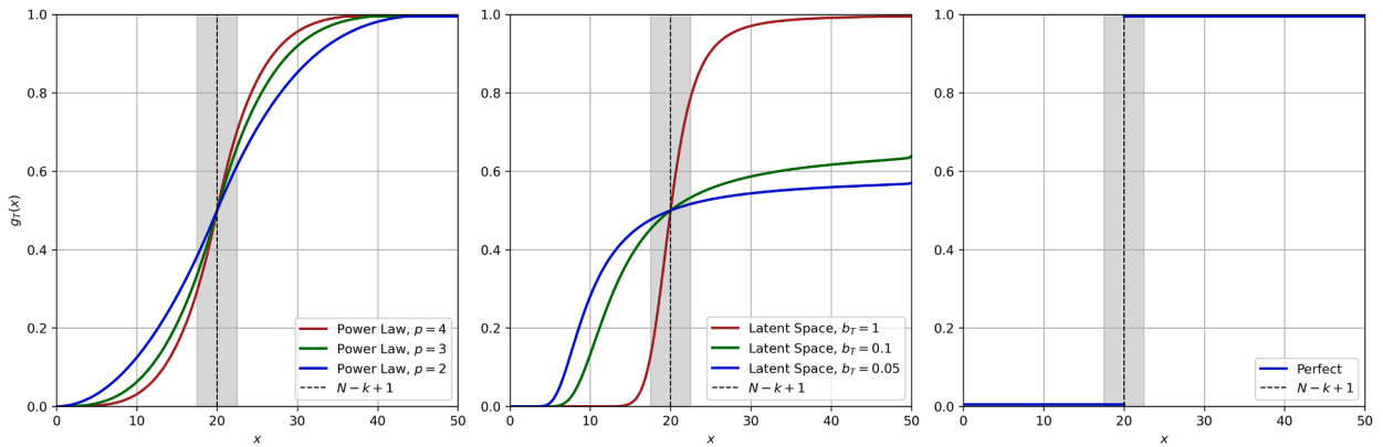
Fig. 2. Representative specifications for g_T . We set N = 50 and k = 31 . In the piecewise power law model, p denotes the power for m < N - k + 1 while the power for m \geq N - k + 1 is chosen automatically to ensure that g_T is smooth. In the latent space model, the distance is specified as d_{ij} = -[\log(1 - (c_{ij}/N)^2)]^{-1} .
