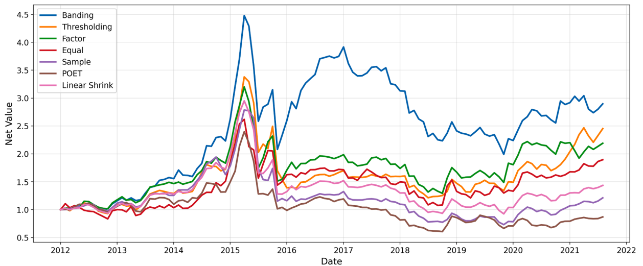
Fig. 5. Out-of-sample mean-variance optimal portfolios. This figure tracks the net value of mean-variance portfolios constructed using different covariance matrix estimation methods. “Thresholding” refers to network-guided thresholding, while “Banding” refers to network-guided banding.
