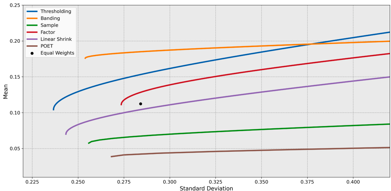
Fig. 4. Out-of-sample efficient frontiers. For the two Network-Guided methods, we show the efficient frontiers using the best auxiliary information. “Thresholding” refers to Network-Guided Thresholding, while “Banding” refers to Network-Guided Banding.
