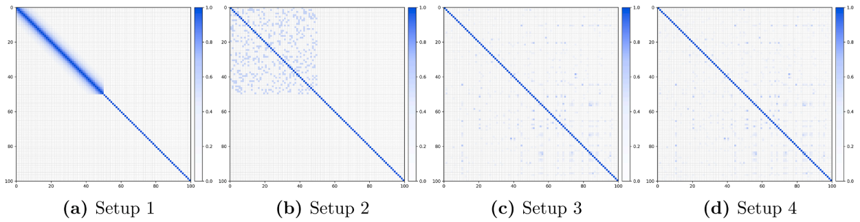
Fig. 3. Typical heatmaps of four data generating processes.
