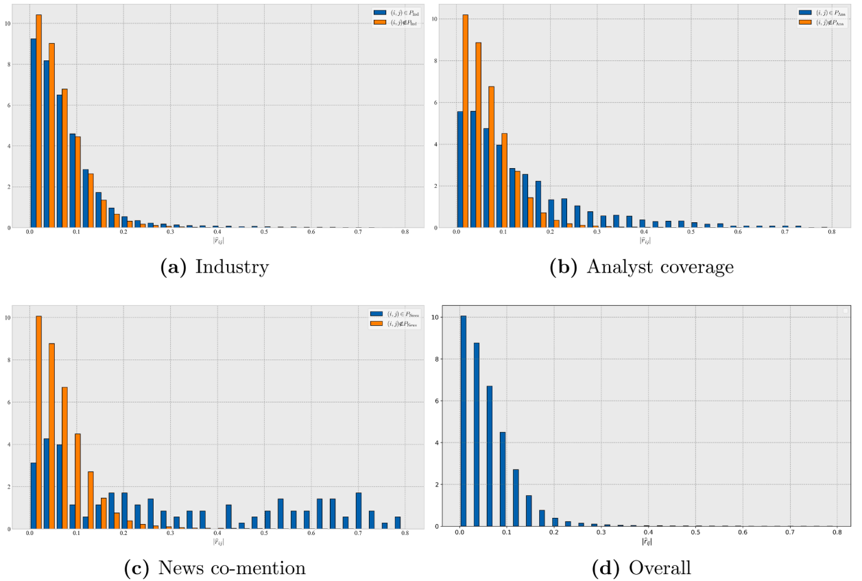
Fig. A.7. Distributions of sample correlations for linked and unlinked pairs. Each panel compares the empirical distributions of sample correlations for entity pairs with a link or without a link as defined by different sources of auxiliary network information.
