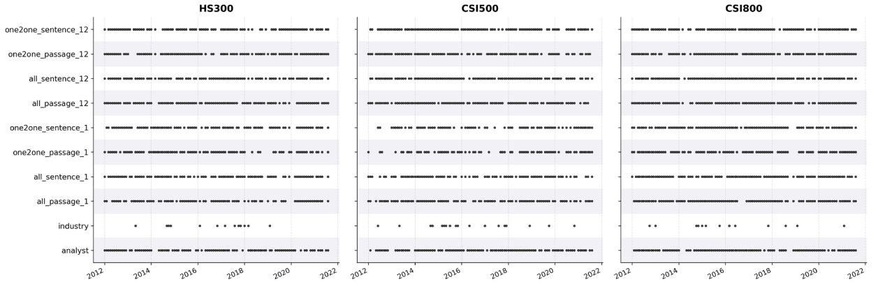
Fig. A.6. Time-varying network usage selected by cross-validation. For each month and each network type on the vertical axis, a dot indicates that cross-validation selects the corresponding network-guided estimator; otherwise, the procedure falls back to the benchmark that ignores the network.
