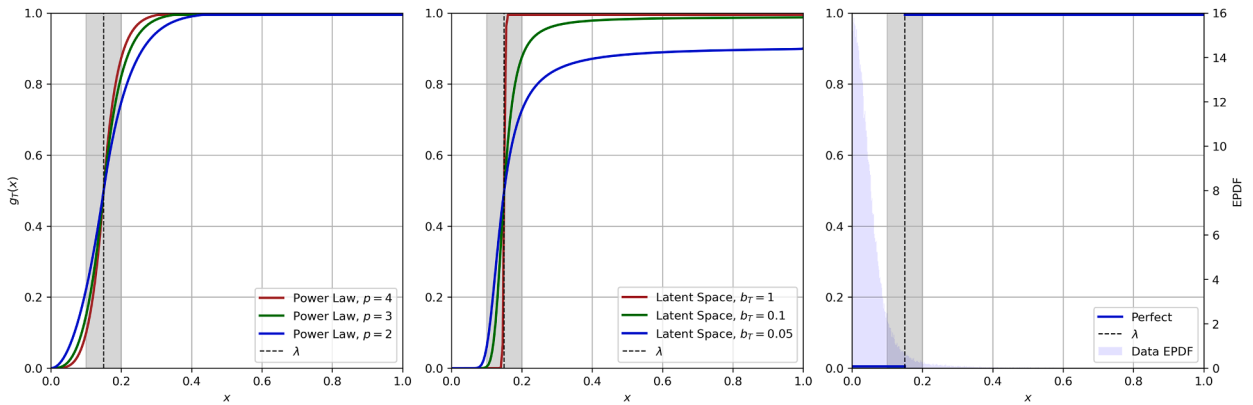
Fig. 1. Representative specifications of g_T . We set \lambda = 0.15 . The (piecewise) power-law family is defined by 0.5x^p I_{\{x \leq \lambda\}} + (1 - 0.5(1-x)^q) I_{\{x > \lambda\}} , with p \in \{2, 3, 4\} where the exponent p applies when x \leq \lambda , while for x > \lambda the power q is chosen automatically to ensure g_T is smooth. The latent-space specification follows (Handcock et al., 2007) and is given by g_T(x) = \frac{\exp\{b_T(d(\lambda) - d(|r_{ij}|))\}}{1 + \exp\{b_T(d(\lambda) - d(|r_{ij}|))\}} , where d(r) = -[\log(1 - r^2)]^{-1} is the inverse Kullback–Leibler divergence distance (see Appendix A.3 for details). The light blue shaded region in the right panel displays the empirical probability density function (EPDF) of the absolute sample correlation between firms' idiosyncratic returns.
